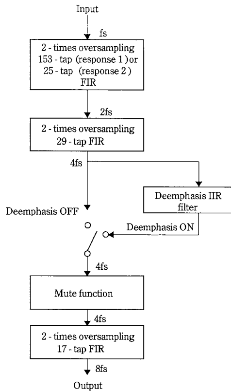
Figure 1. Arithmetic block diagram
