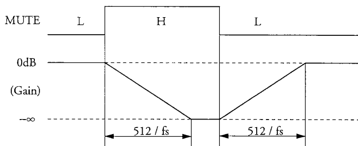
Figure 2. Mute timing
