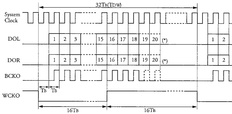
Figure 11. 18/20-bit output ( \overline{CKSL} = \text{LOW} )
