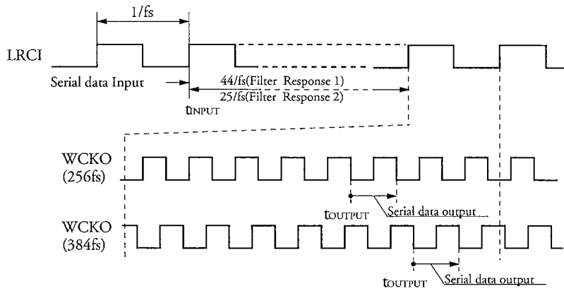
Figure 12. Delay timing (SYNCN = LOW)
