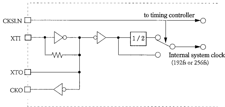
Figure 5. Clock generator circuit
